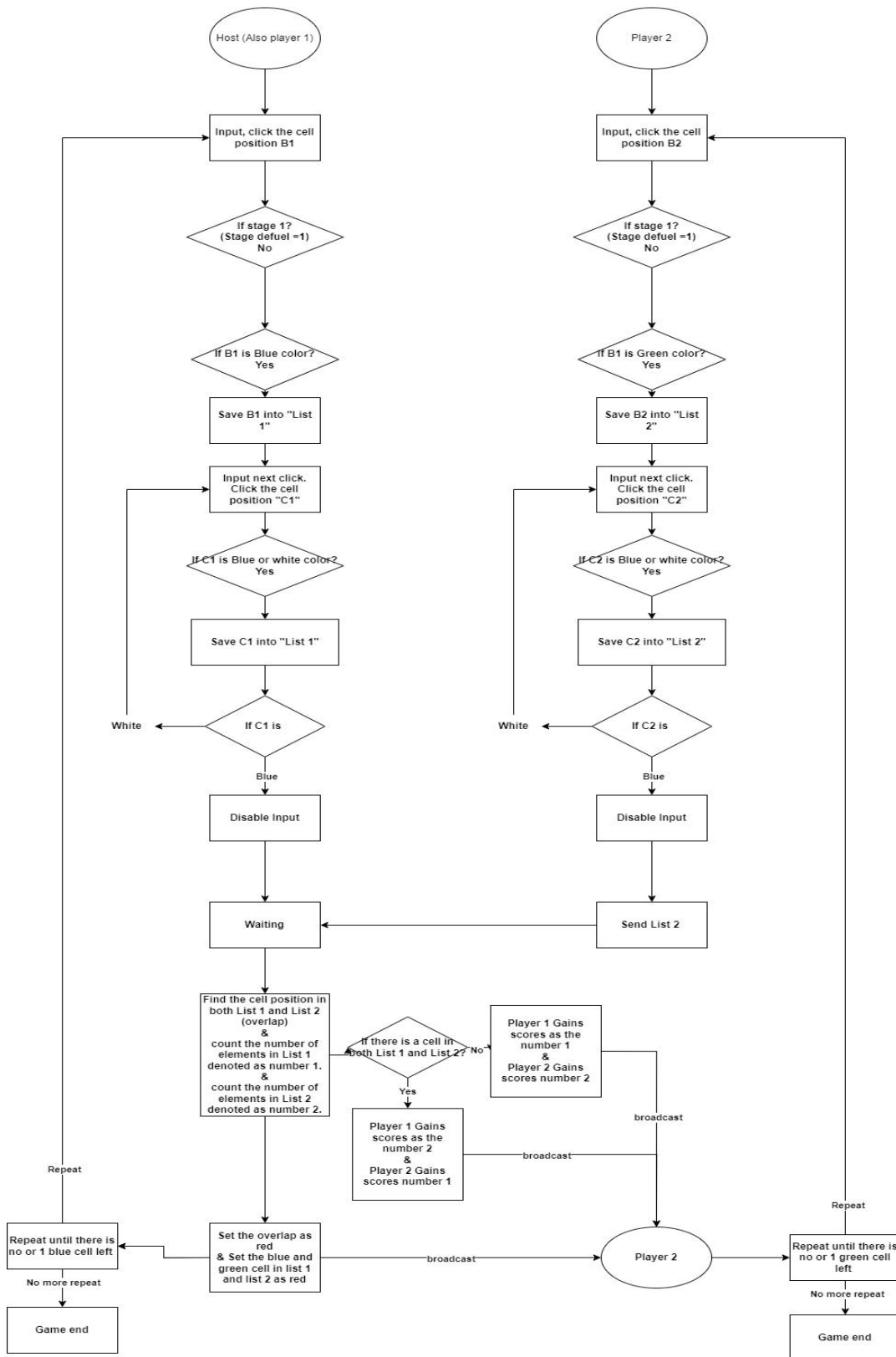
Figure A1. Flow chart of game logic.
